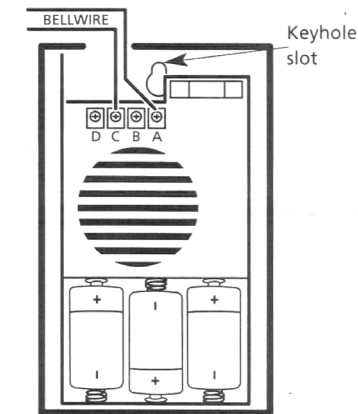
Circuit Diagram for normal bell push
